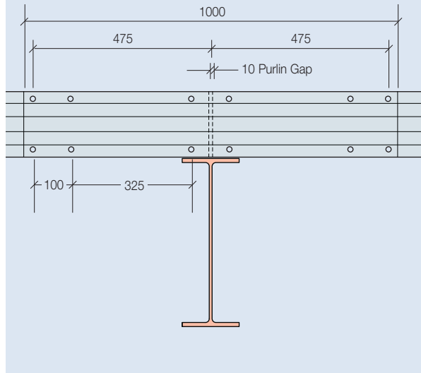
Sleeve Hole Dimensions
