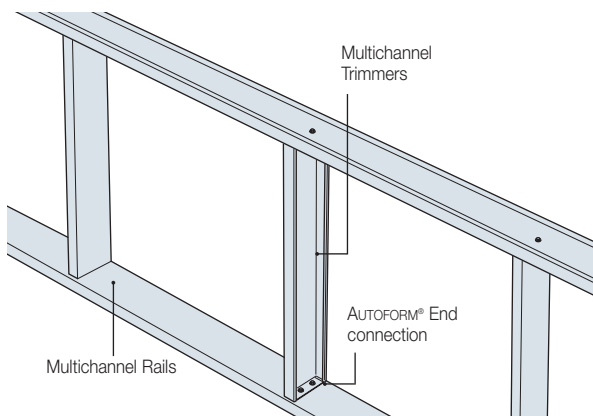
Window Trimmers
