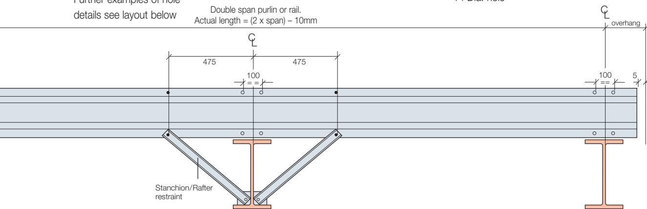
RAFTER/STANCHION STAY HOLES (See above)
